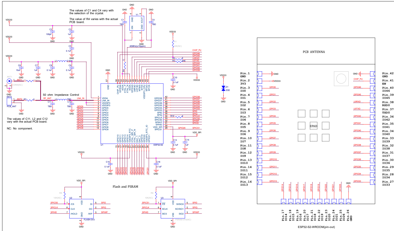
Figure 5: ESP32-S2-WROOM Schematics
