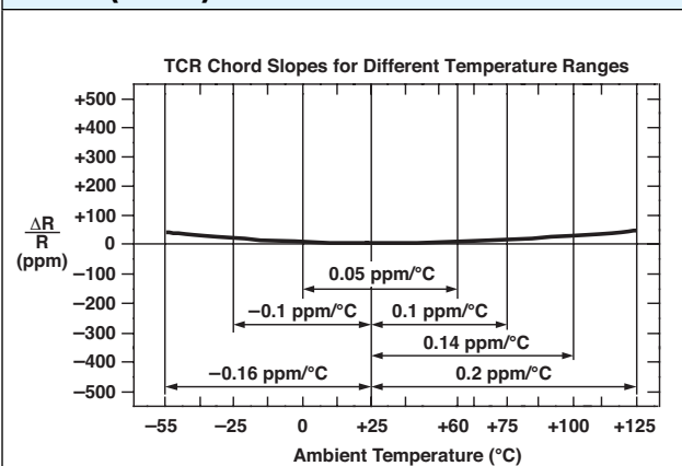
Figure 5 – Typical Resistance/Temperature Curve (Z-Foil)
