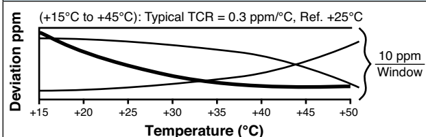
Figure 4 – Typical Curves Within 10 ppm Window, VHP10x Laboratory Instrument Range
