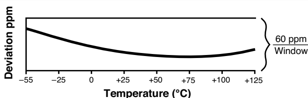
Figure 1 – A Typical VHP10x Resistance Temperature Curve
