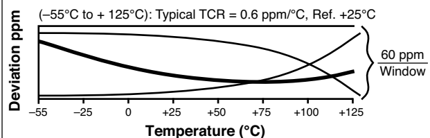
Figure 3 – Typical Curves Within the 60 ppm Window, VHP10x TCR for Mil Range
