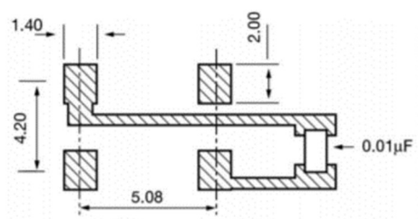
Figure 5) Top, Side, Bottom views and Suggested Land
