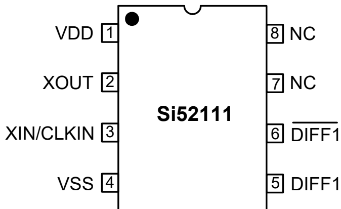
Figure 7. 8-Pin TSSOP
