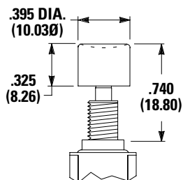
L Plunger with Cap P/N 8941
