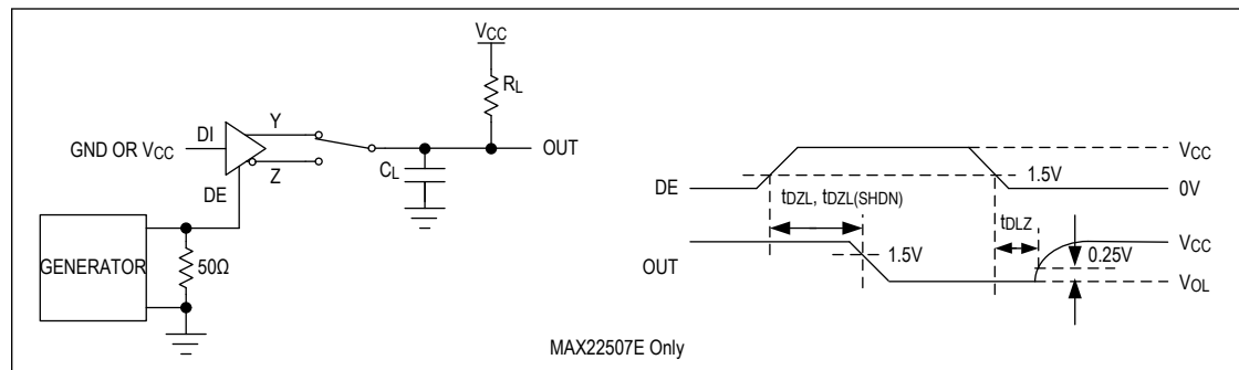
Figure 5. Driver Enable and Disable Times ( t_{DLZ} , t_{DLZ} )
