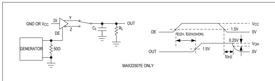
Figure 4. Driver Enable and Disable Times ( t_{DZH} , t_{DZH} )
