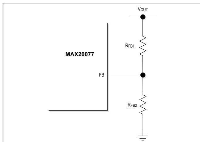
Figure 1. Adjustable Output-Voltage Setting
