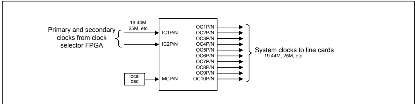
Figure 1-1. Telecom Timing Card
