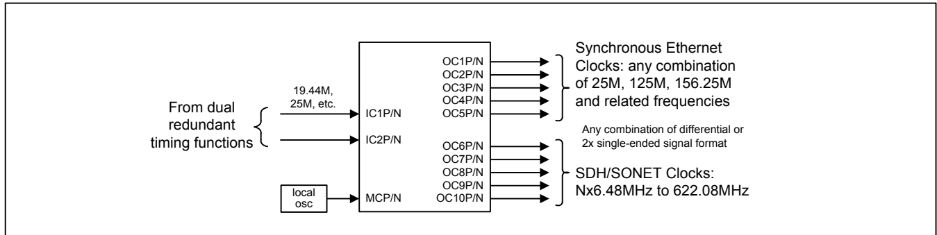
Figure 1-2. Synchronous Ethernet and SDH/SONET Line Card
