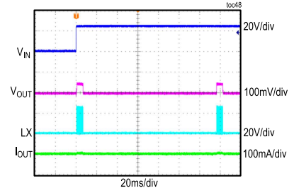
MAX17640B OUTPUT SHORT DURING STARTUP FIGURE 6 CIRCUIT
