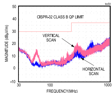
MAX17640B RADIATED EMISSIONS PLOT
