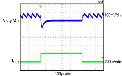
MAX17640A LOAD TRANSIENT RESPONSE FIGURE 5 CIRCUIT
