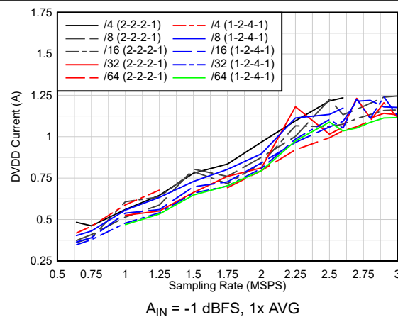
Figure 6-103. Current vs Sampling Rate vs Real Decimation
