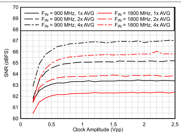
Figure 8-3. SNR vs Clock Amplitude (dither off)
