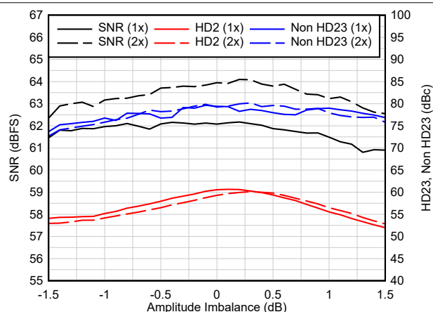
Figure 7-5. Amplitude Imbalance - 3.0 GSPS
