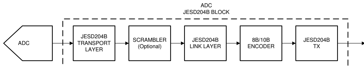
Figure 7-41. JESD204B Block Diagram
