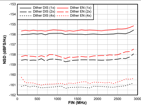
Figure 6-83. AC Performance vs F_{IN}
