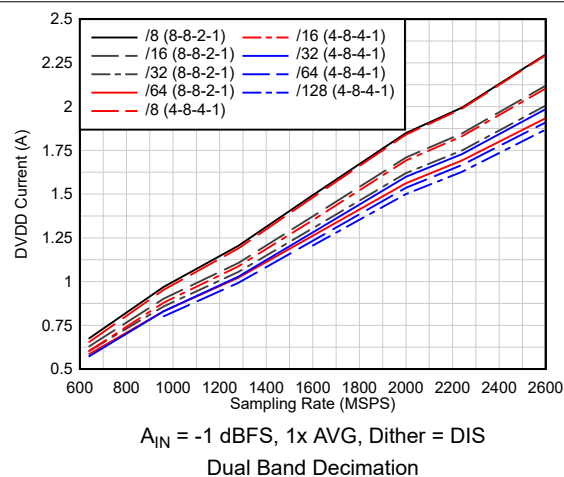
Figure 6-52. Current vs Sampling Rate vs Decimation
