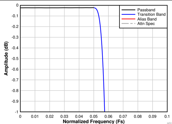
Figure 7-27. Decimation by 8 Passband Ripple Response
