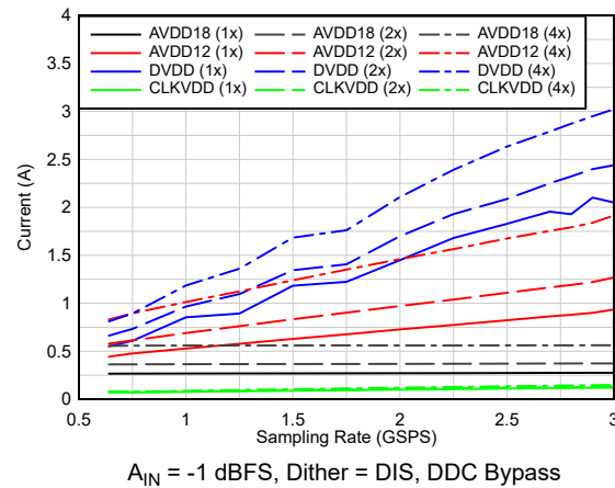
Figure 6-101. Current vs Sampling Rate vs Averaging
