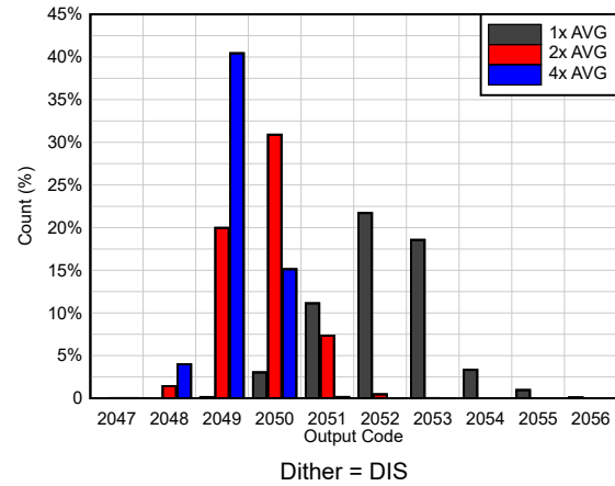
Figure 6-99. DC Offset Histogram
