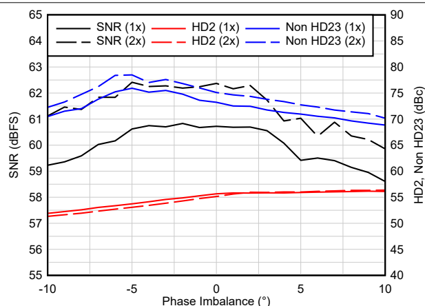
Figure 7-6. Phase Imbalance - 3.0 GSPS
