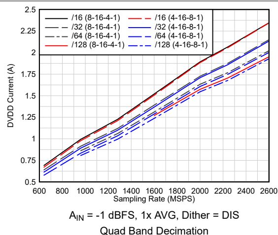
Figure 6-54. Current vs Sampling Rate vs Decimation
