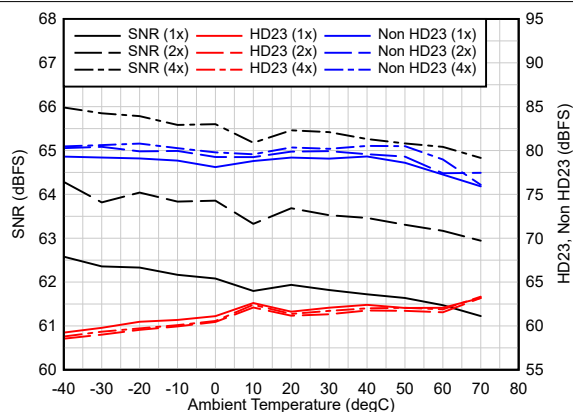
Figure 6-93. AC Performance vs Temperature
