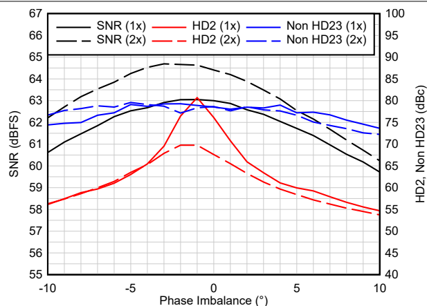
Figure 7-4. Phase Imbalance - 2.6 GSPS
