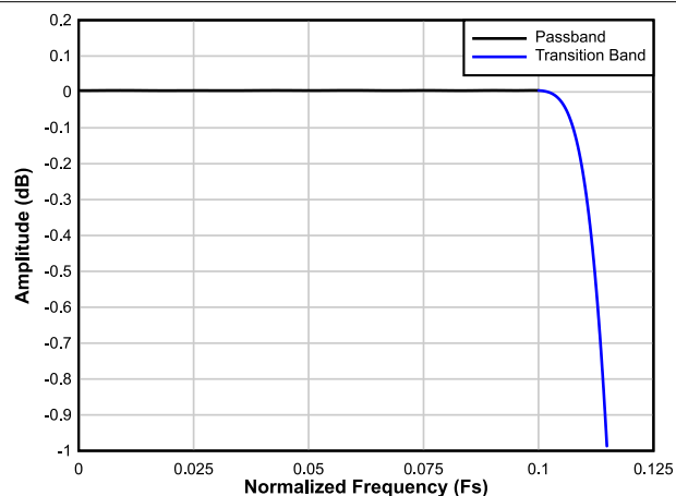
Figure 7-25. Decimation by 4 Passband Ripple Response
