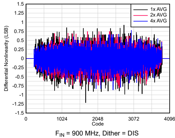
Figure 6-98. DNL vs Code
