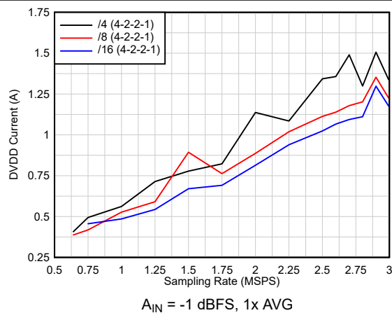
Figure 6-102. Current vs Sampling Rate vs Real Decimation
