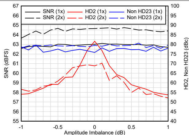
Figure 7-3. Amplitude Imbalance - 2.6 GSPS
