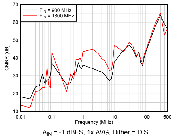
Figure 6-100. CMRR
