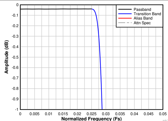
Figure 7-29. Decimation by 16 Passband Ripple Response
