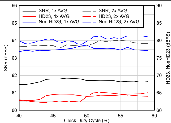
Figure 6-95. AC Performance vs Clock Duty Cycle
