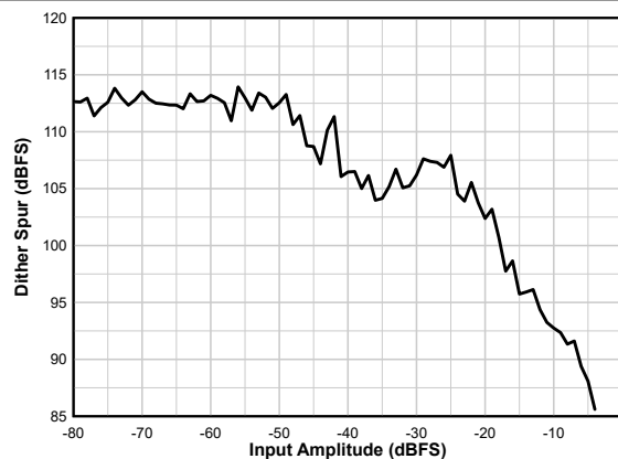
F_{IN} = 900 MHz,
