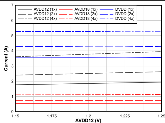
Figure 6-111. I_{AVDD12} vs Supply
