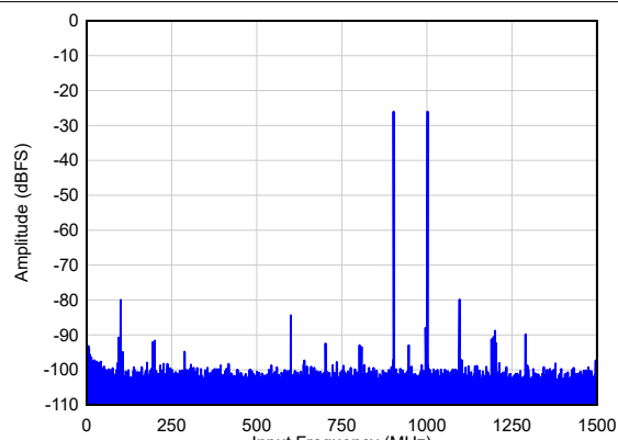
Figure 6-80. Two Tone FFT at F_{IN} = 900/1000 MHz
