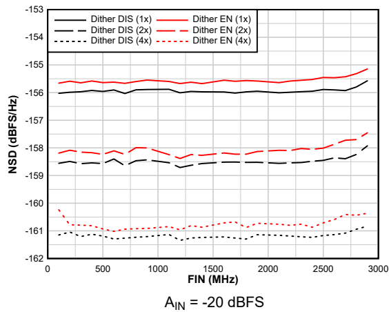
Figure 6-31. NSD Performance vs F_{IN}
