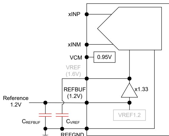
The ADC3644 is equipped with an on-chip reference buffer that also includes gain to generate the 1.6 V reference voltage from an external 1.2 V reference. A 10 \mu F and a 0.1 \mu F ceramic bypass capacitor ( C_{VREF} ) between the VREF and REFGND pins and a 10 \mu F and a 0.1 \mu F ceramic bypass capacitor between the REFBUF and REFGND pins are recommended. Both capacitors should be placed as close to the pins as possible. The load current from the external reference is less than 100 \mu A.
