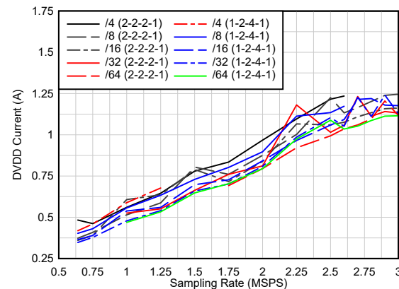
Figure 6-101. Current vs Sampling Rate vs Averaging
