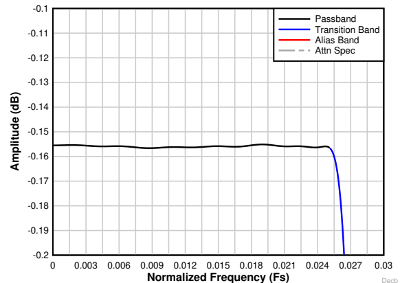
Figure 8-28. Decimation by 16 complex passband ripple response
