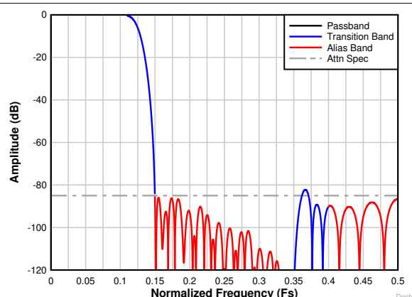
Figure 8-23. Decimation by 4 complex frequency response
