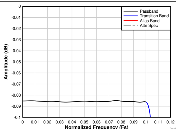
Figure 8-24. Decimation by 4 complex passband ripple response
