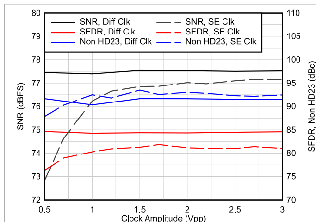
Figure 8-8. AC Performance vs Clock Amplitude for F_{IN} = 5 MHz
