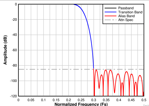
Figure 8-21. Decimation by 2 complex frequency response
