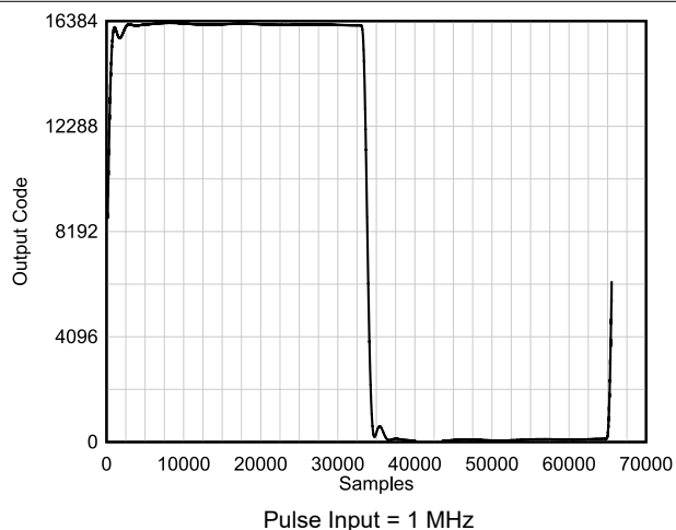
Figure 6-26. Pulse Response
