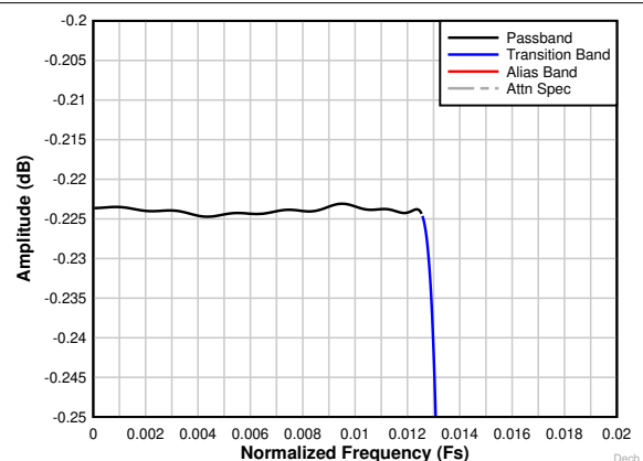
Figure 8-30. Decimation by 32 complex passband ripple response
