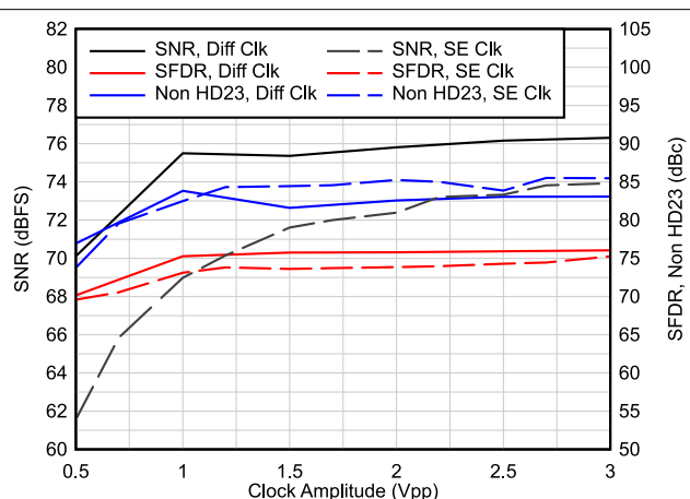
Figure 8-9. AC Performance vs Clock Amplitude for F_{IN} = 70 MHz
