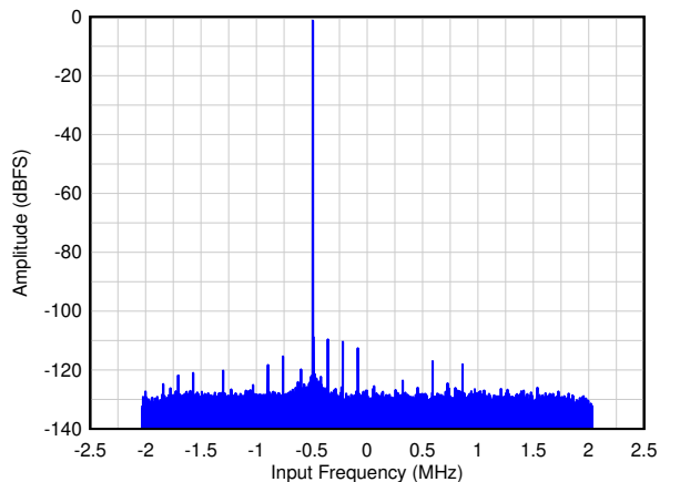
Figure 9-3. Single Tone FFT at F_{IN} = 5 MHz
