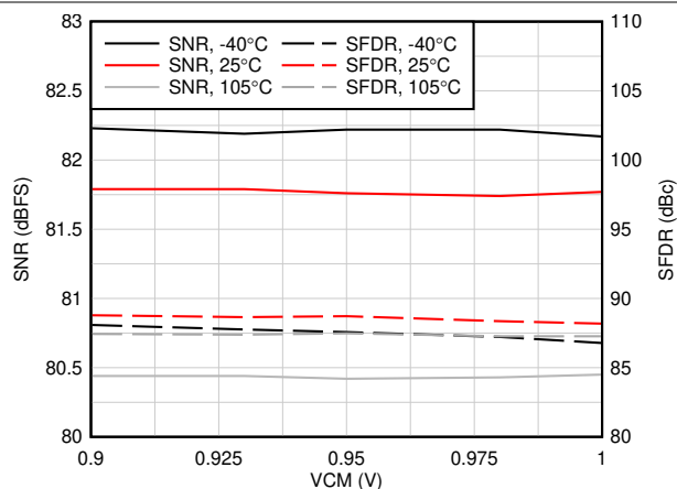
Figure 6-18. AC Performance vs VCM vs Temperature
