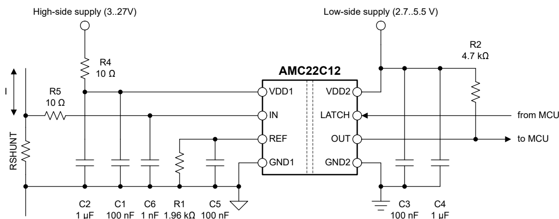
Figure 8-6. Decoupling of the AMC22C12
