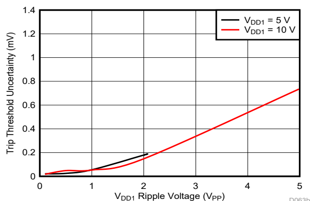
Figure 8-5. Trip Threshold Sensitivity to VDD1 Ripple Voltage (Cmp1, f_{\text{RIPPLE}} = 10 kHz)
