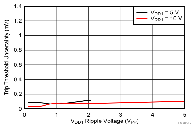
Figure 8-4. Trip Threshold Sensitivity to VDD1 Ripple Voltage (Cmp0, f_{\text{RIPPLE}} = 10 kHz)
