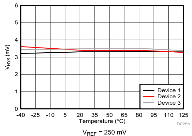
Figure 6-16. Cmp0 Trip Threshold Hysteresis vs Temperature
