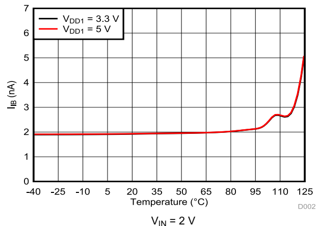
Figure 6-40. Input Bias Current vs Temperature
