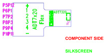
Figure 24. ADT7320FBZ Silkscreen
