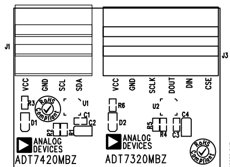
Figure 21. ADT7x20 Evaluation Board External Board Silkscreen
