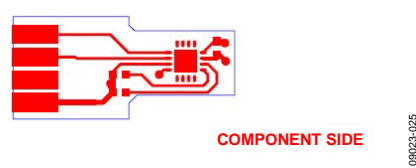
Figure 25. ADT7420FBZ Component Side (Layer 1)
