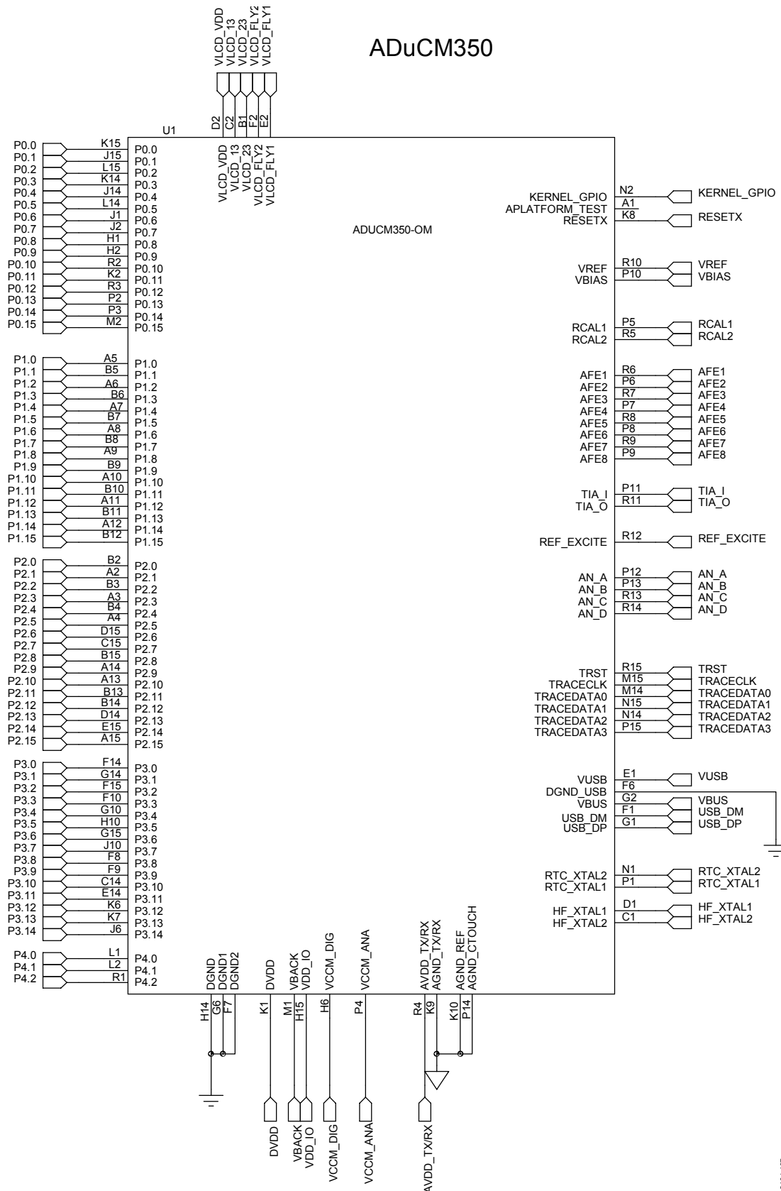
Figure 7. ADuCM350 Motherboard Schematic Device Drawing
