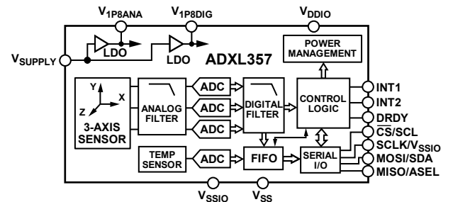
Figure 2. ADXL357
