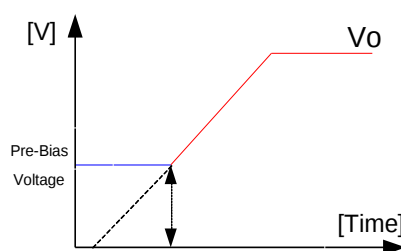
Figure 11: Pre-Bias startup
