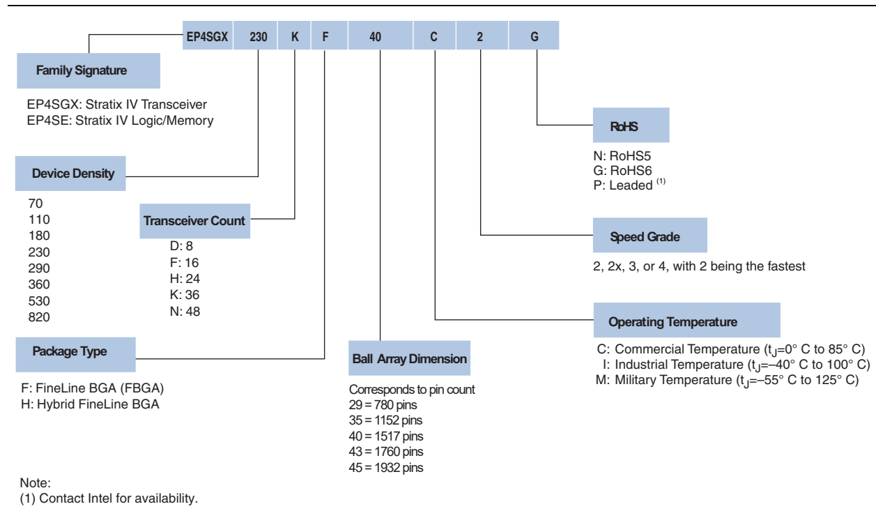
Figure 1-4. Stratix IV GX and E Device Packaging Ordering Information
