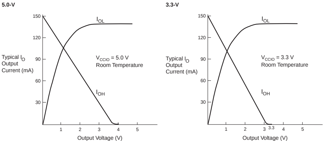
Figure 13. Output Drive Characteristics of MAX 9000 Devices
