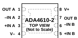
Figure 5. ADA4610-2 Pin Configuration, 8-Lead MSOP (RM Suffix)
