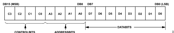
Figure 2. Input Shift Register Contents
