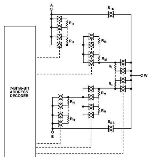
Figure 36. AD5123/AD5143 Simplified RDAC Circuit
