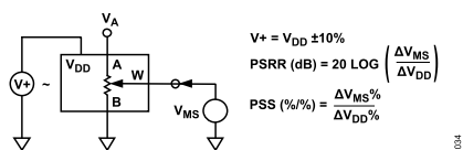
Figure 34. Power Supply Sensitivity and Power Supply Rejection Ratio (PSS, PSRR)
