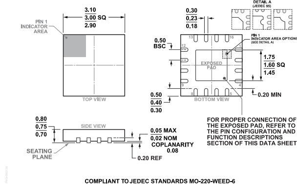
Figure 41. 16-Lead Lead Frame Chip Scale Package [LFCSP] 3 mm × 3 mm Body and 0.75 mm Package Height (CP-16-22) Dimensions shown in millimeter
