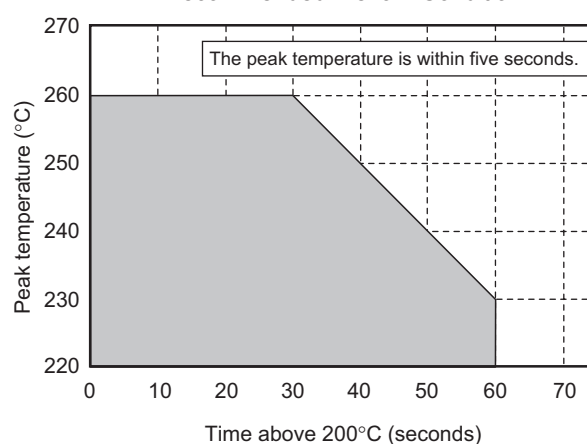
Recommended Reflow Condition
