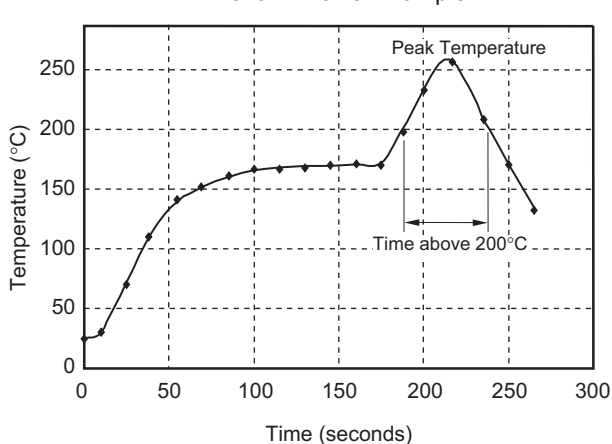
Reflow Profile Example
