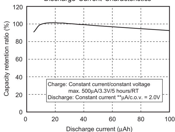
Discharge Current Characteristics
