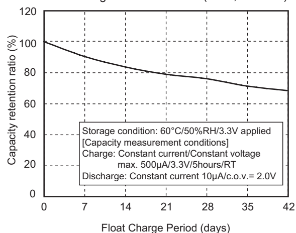
Float-Charge Characteristics (60°C, 50%RH)
