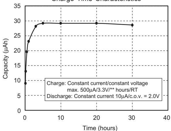
Charge Time Characteristics
