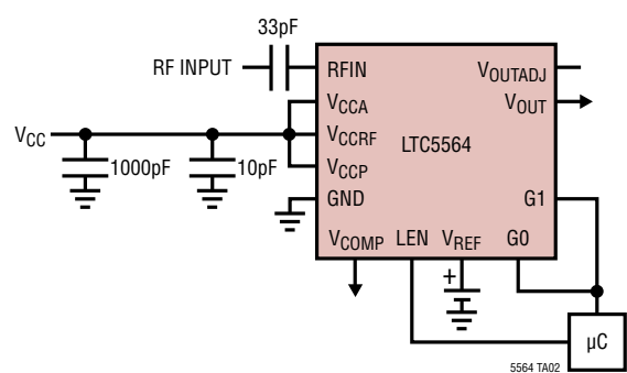
600MHz to 15GHz RF Power Detector
