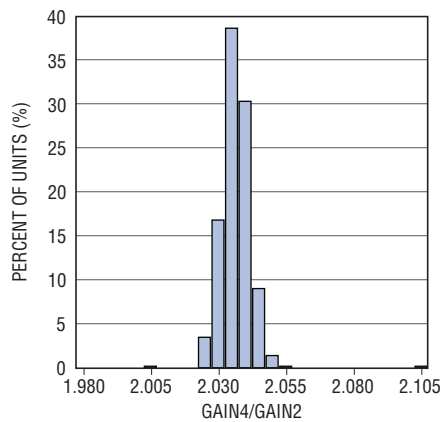
GAIN4/GAIN2 Histogram
