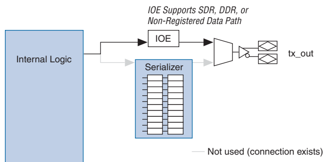
Figure 5–5. Serializer Bypass
